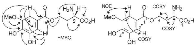
Scheme 2. Aleurodiscoester ( 2 ) with selected HMBC, COSY, and ROESY correlations.
