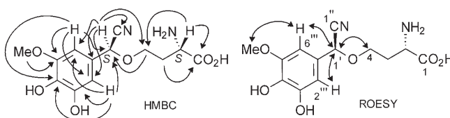
Scheme 1. Aleurodisconitrile ( 1 ) with selected HMBC and ROESY correlations.
