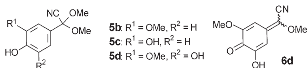
Scheme 4. Oxidation products of the model compounds 3b–d .
