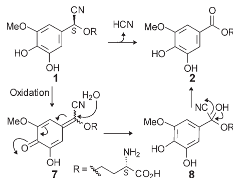
Scheme 5. Proposal for the oxidative degradation of 1 to 2 .
