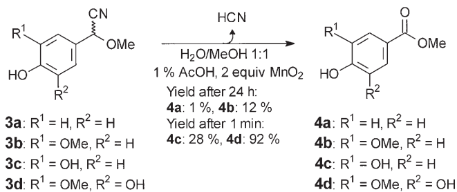
Scheme 3. Oxidative degradation of the model compounds 3a–d to the corresponding esters 4a–d by release of HCN.
